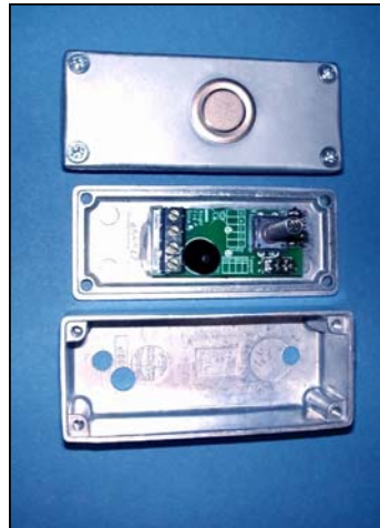
Fig. 2 – Z40 Final Exit Set Switch
