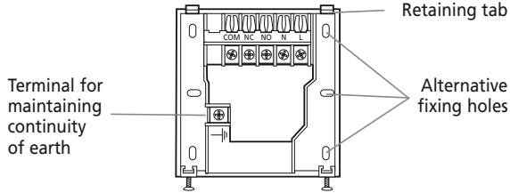
Fig. 4 Mount the wall plate in this configuration only
