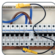
2 long and 2 short leads for 'dead' testing (insulation & R_1 + R_2 testing)
