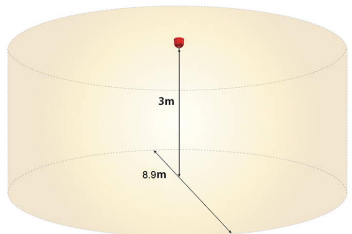
EN54-23 Coverage: C-3-8.9
